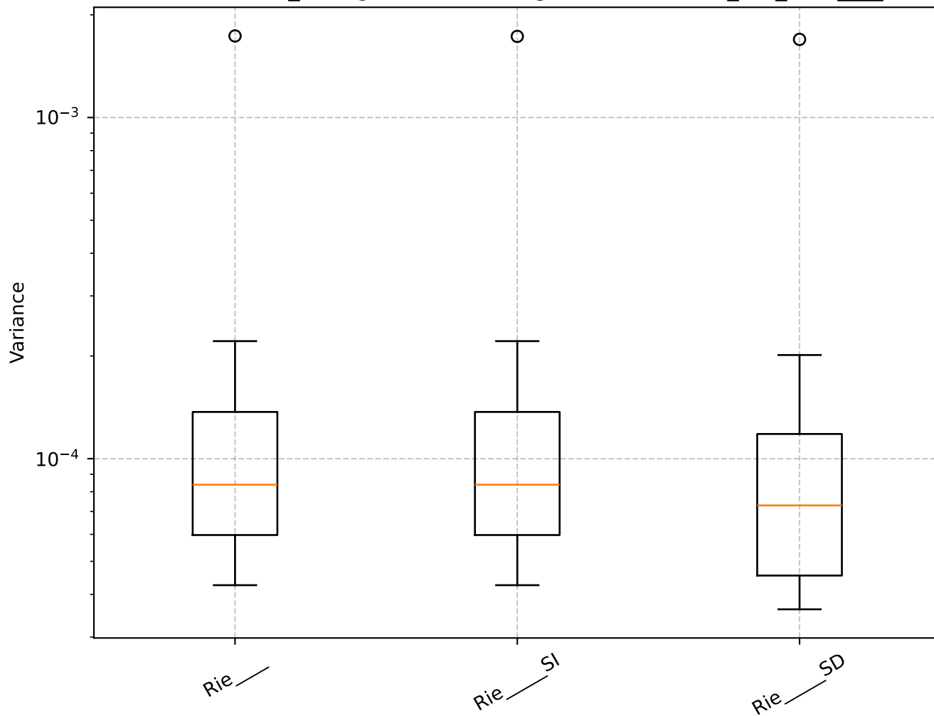
Q=0.71, len_rolling=100: Shrinkage Box Plot - min_var_, Rie____
