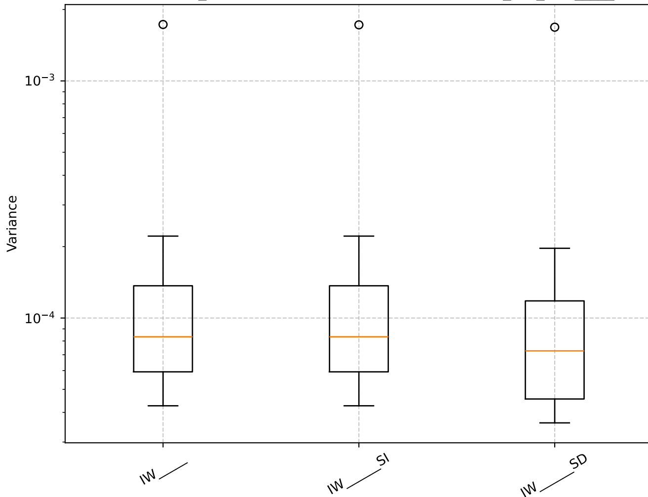
Q=0.75, len_rolling=100: Shrinkage Box Plot - min_var_, IW_____
