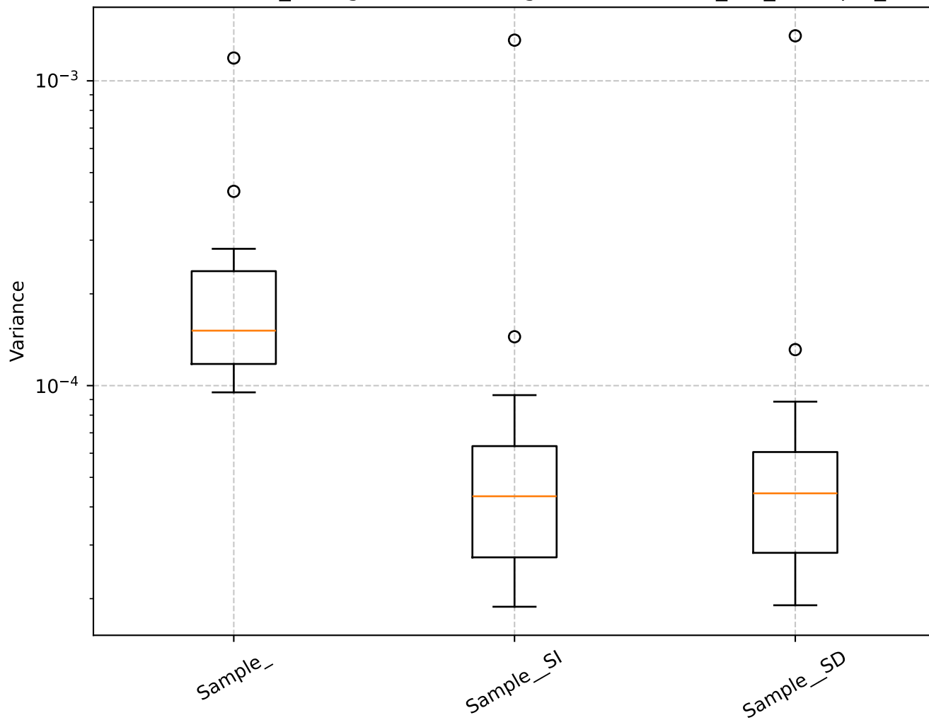
Q=0.75, len_rolling=100: Shrinkage Box Plot - min_var_, Sample_
