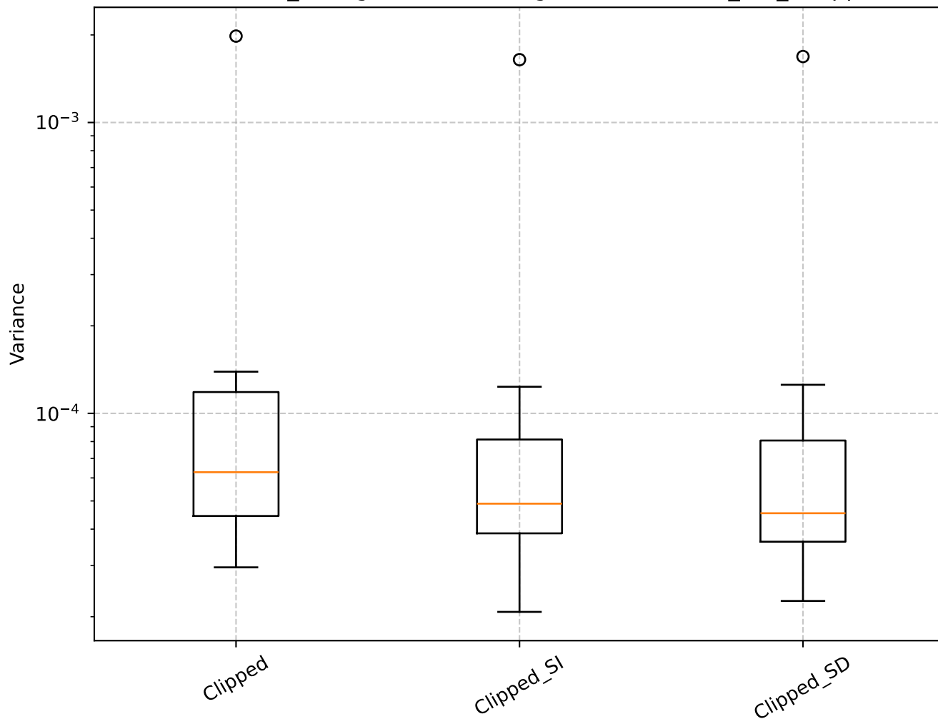
Q=0.77, len_rolling=100: Shrinkage Box Plot - min_var_, Clipped
