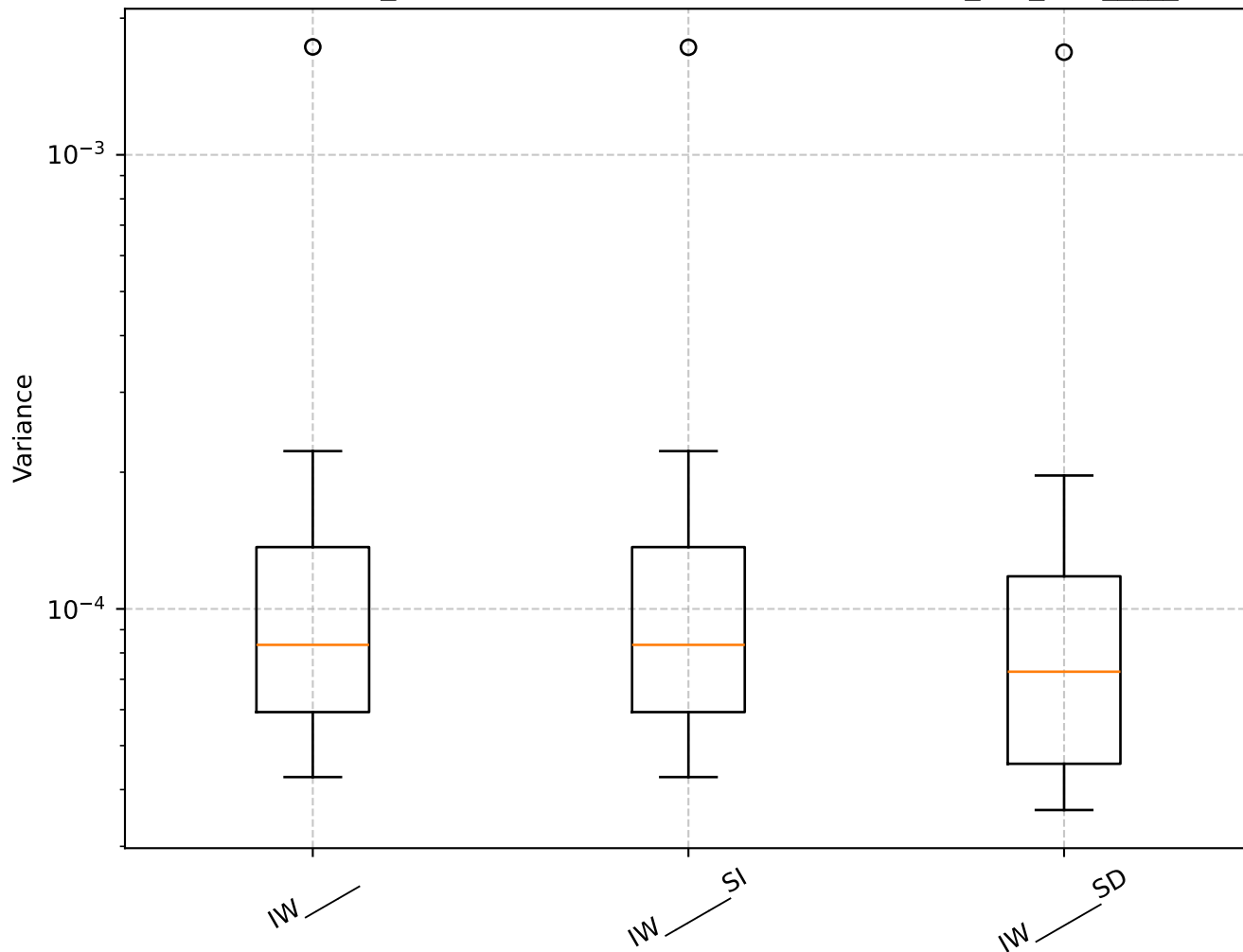
Q=0.77, len_rolling=100: Shrinkage Box Plot - min_var_, IW_____
