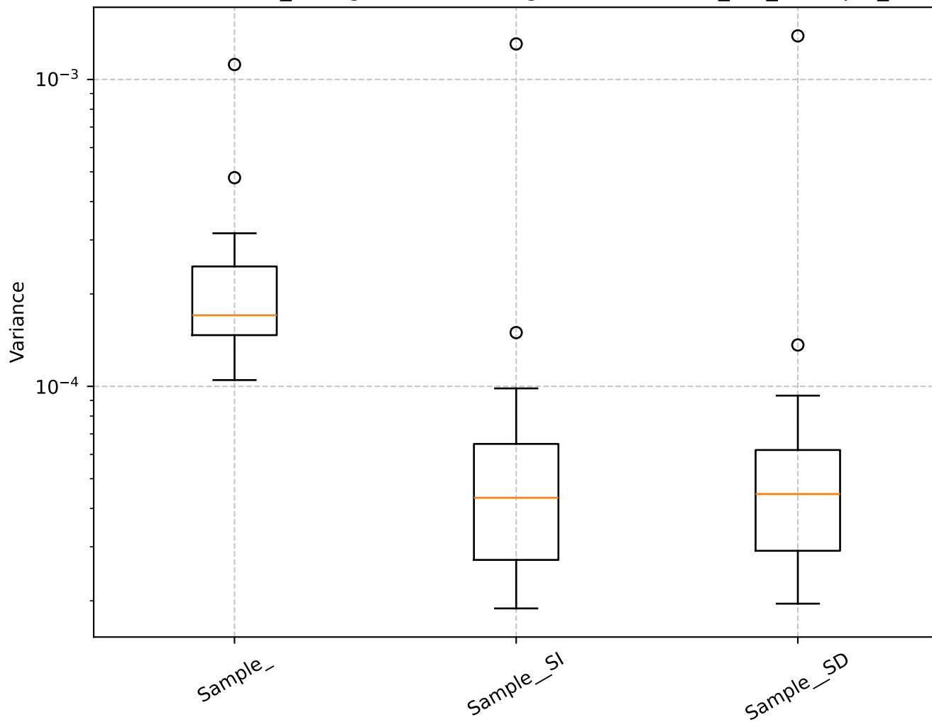
Q=0.78, len_rolling=100: Shrinkage Box Plot - min_var_, Sample_
