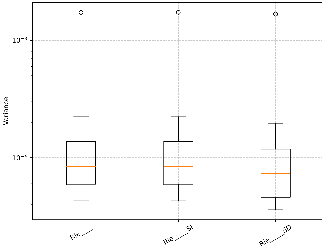
Q=0.80, len_rolling=100: Shrinkage Box Plot - min_var_, Rie____
