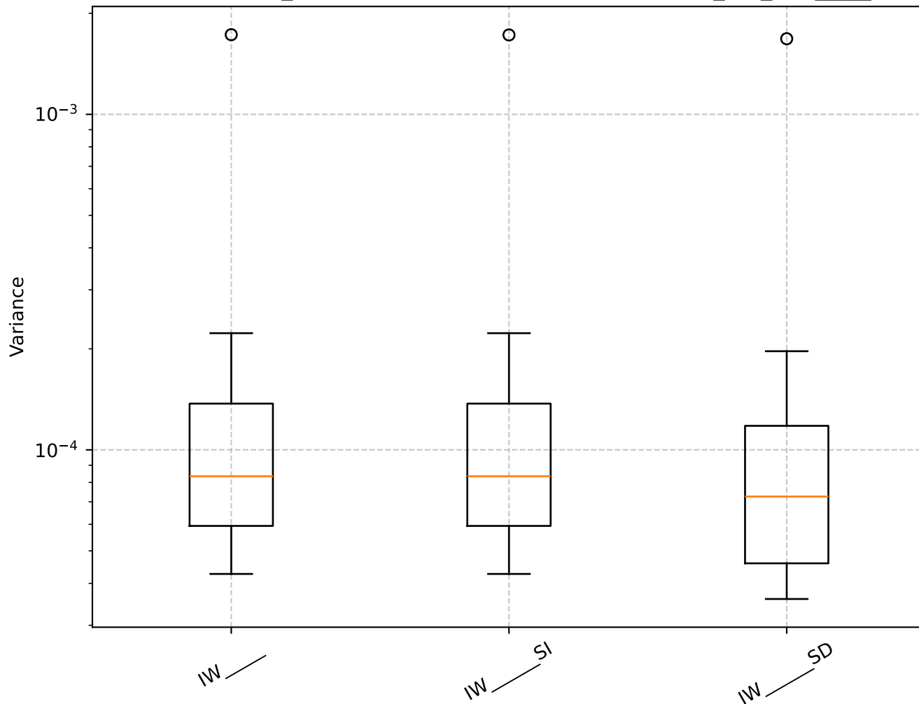
Q=0.82, len_rolling=100: Shrinkage Box Plot - min_var_, IW_____
