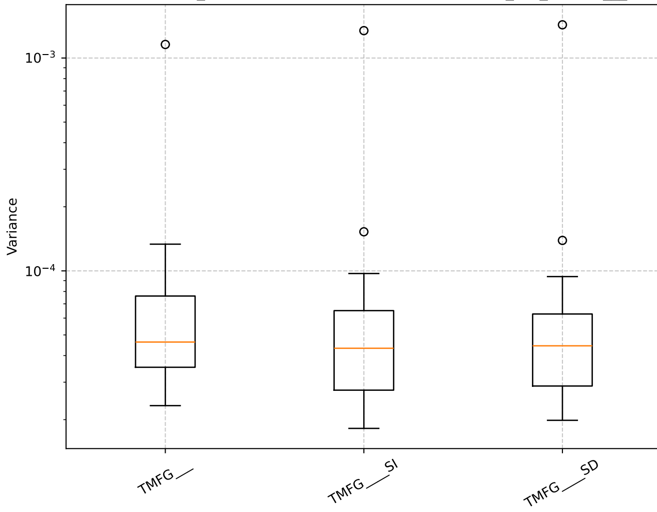
Q=0.82, len_rolling=100: Shrinkage Box Plot - min_var_, TMFG__
