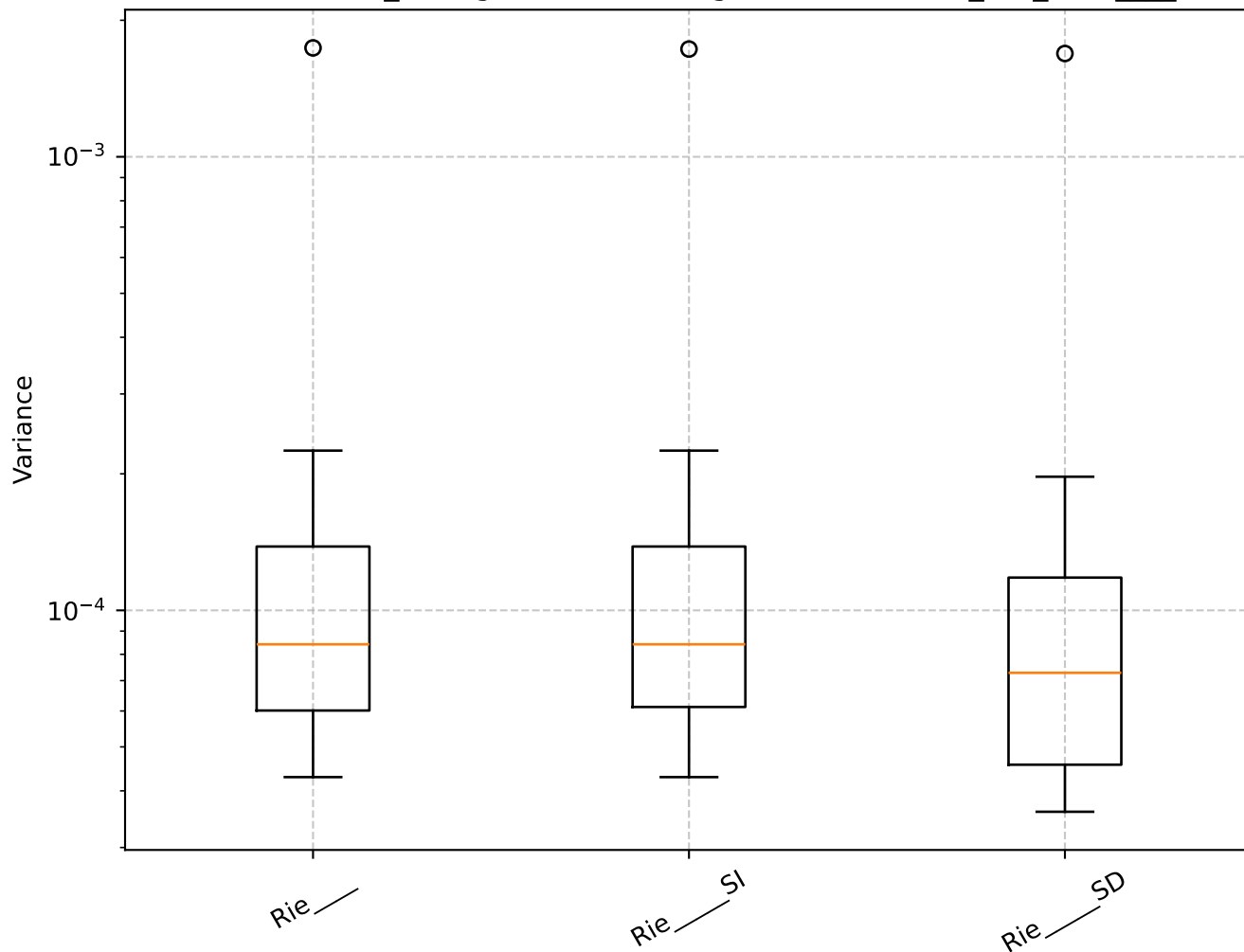
Q=0.87, len_rolling=100: Shrinkage Box Plot - min_var_, Rie____
