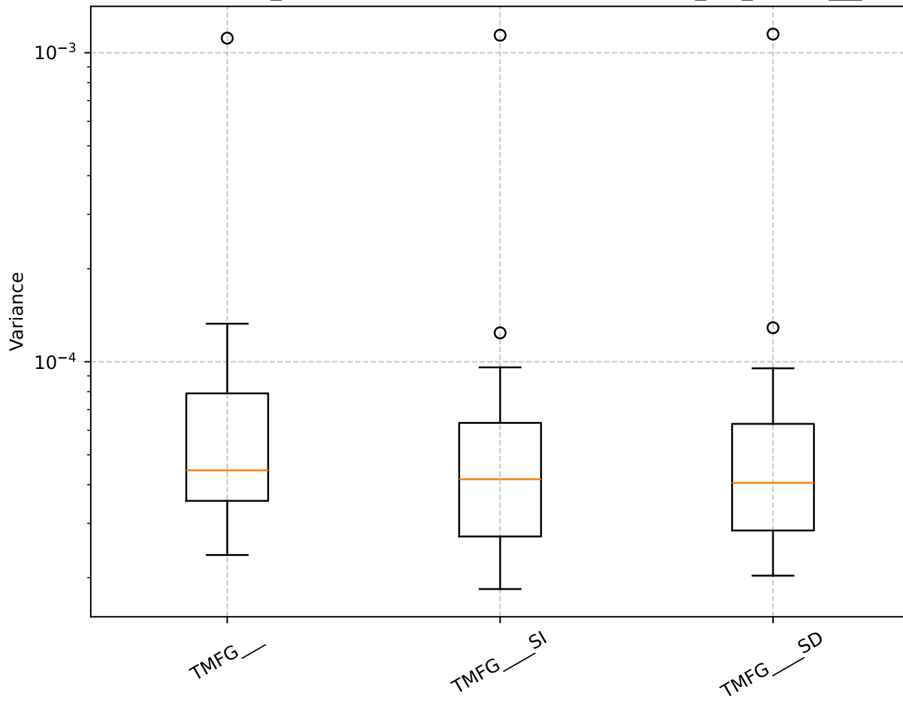
Q=0.91, len_rolling=100: Shrinkage Box Plot - min_var_, TMFG__
