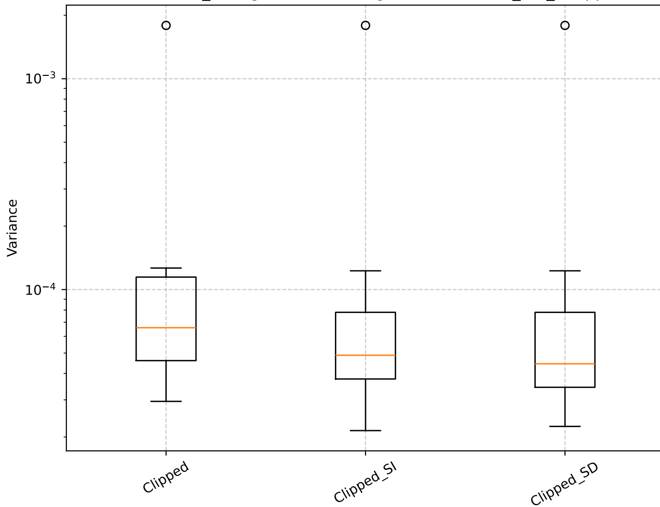
Q=0.95, len_rolling=100: Shrinkage Box Plot - min_var_, Clipped
