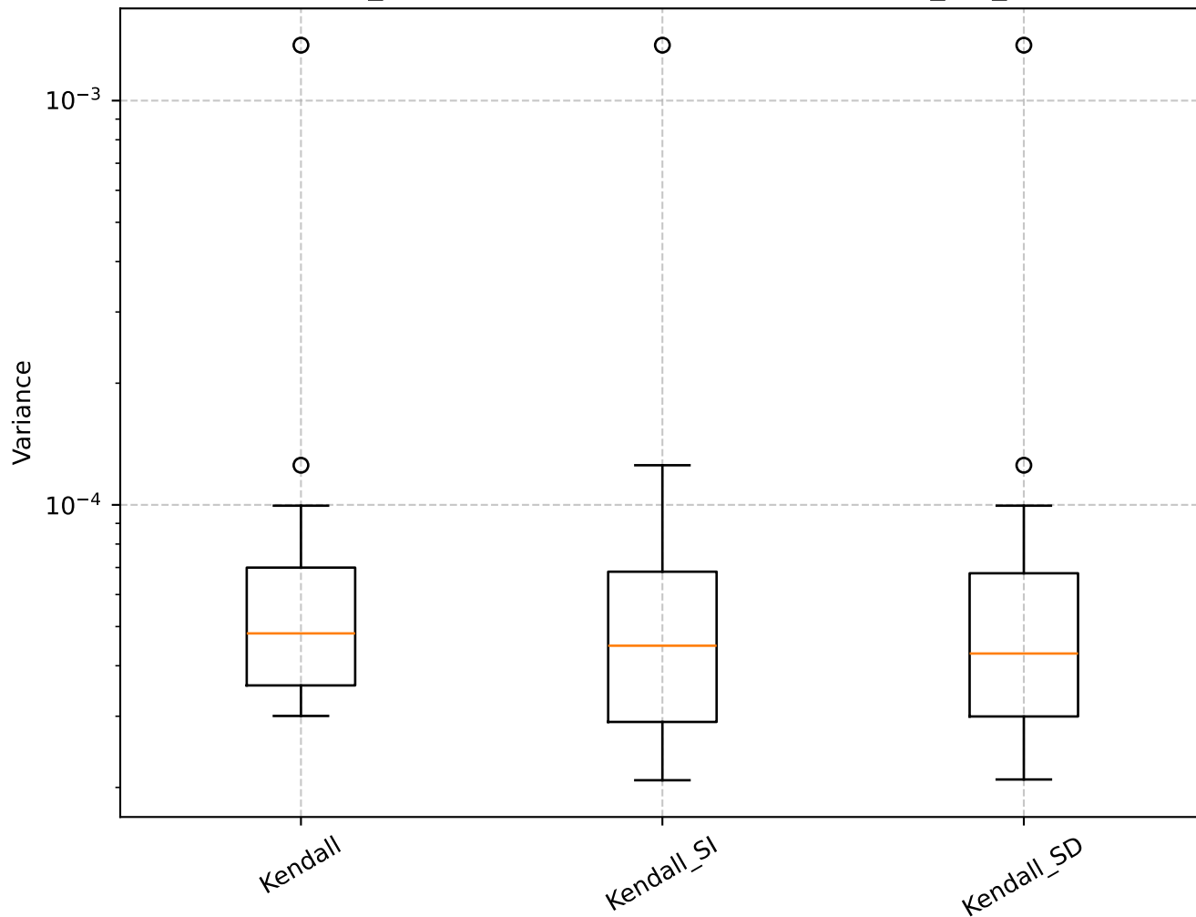
Q=0.95, len_rolling=100: Shrinkage Box Plot - min_var_, Kendall
