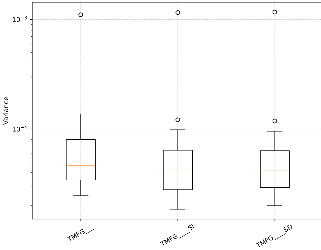
Q=0.95, len_rolling=100: Shrinkage Box Plot - min_var_, TMFG__
