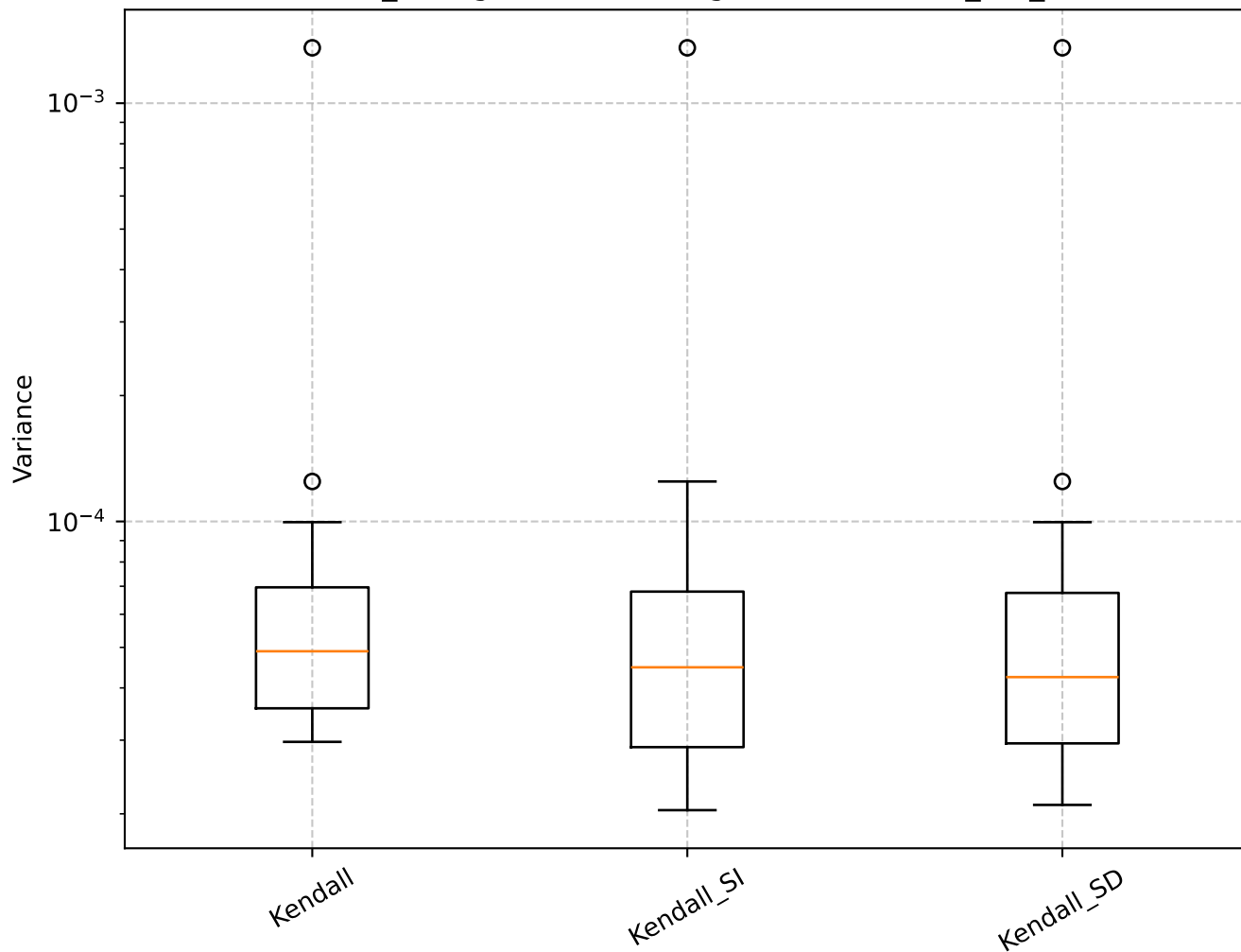
Q=0.98, len_rolling=100: Shrinkage Box Plot - min_var_, Kendall
