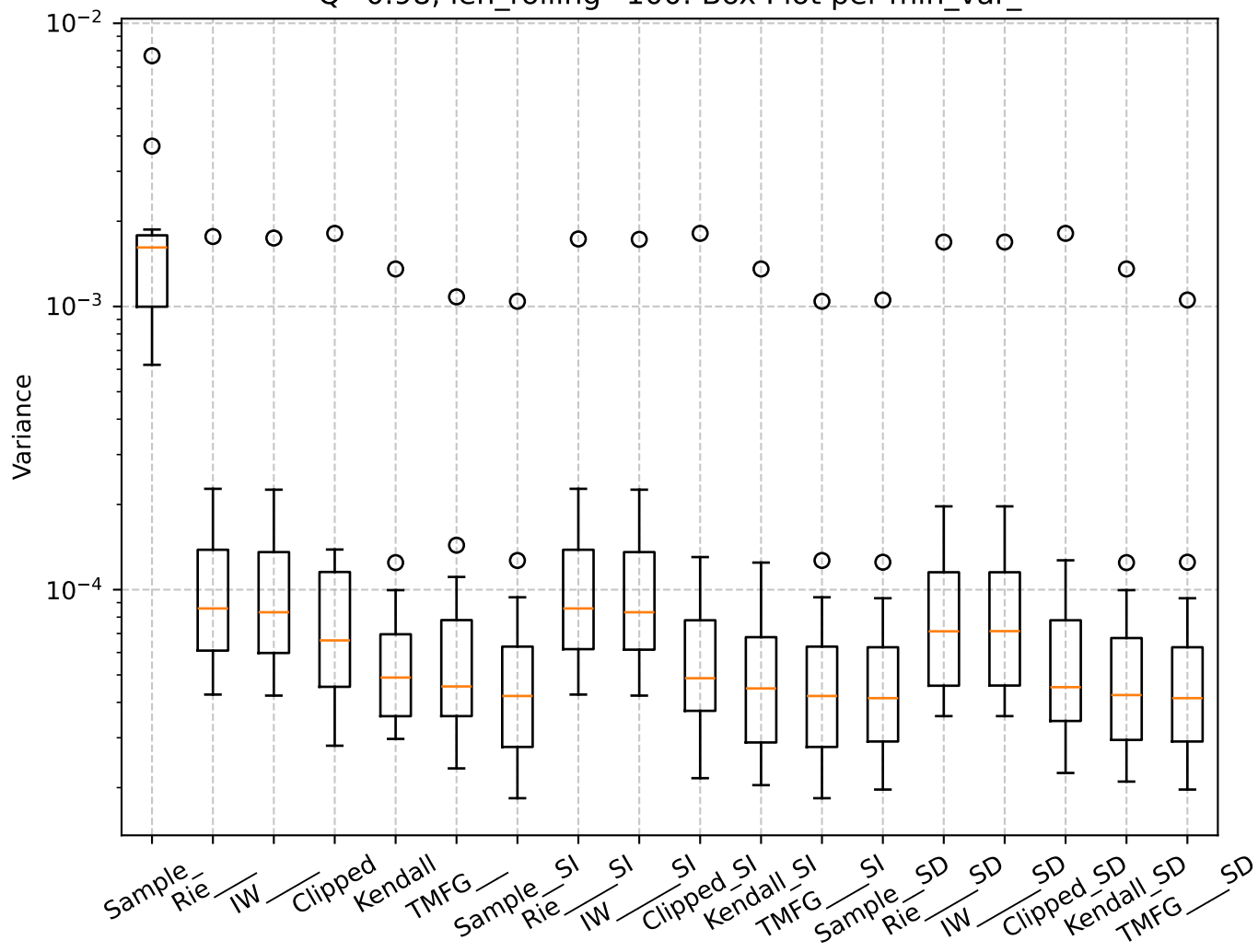
Q=0.98, len_rolling=100: Box Plot per min_var_
