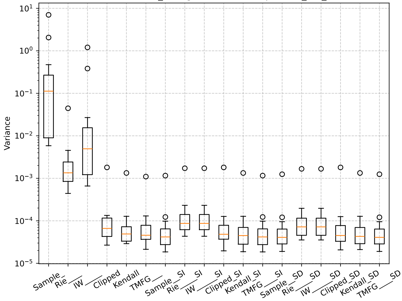
Q=1.05, len_rolling=100: Box Plot per min_var_
