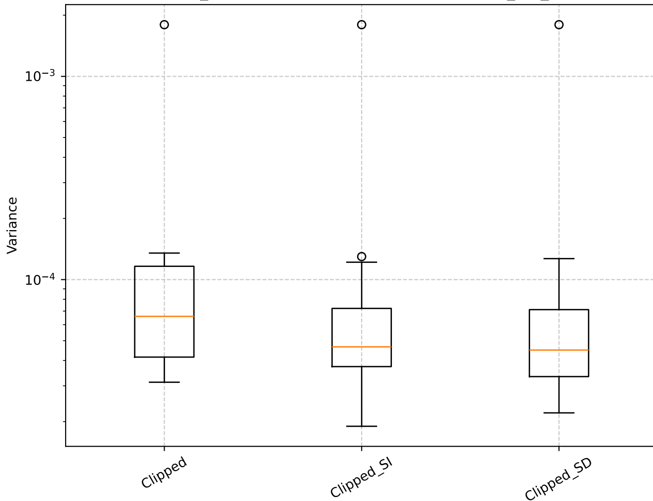
Q=1.11, len_rolling=100: Shrinkage Box Plot - min_var_, Clipped
