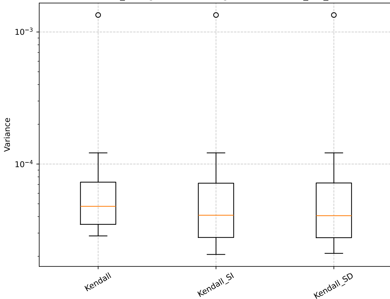
Q=1.21, len_rolling=100: Shrinkage Box Plot - min_var_, Kendall
