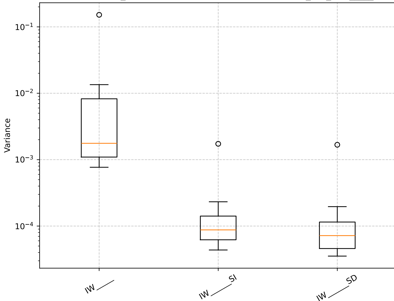
Q=1.25, len_rolling=100: Shrinkage Box Plot - min_var_, IW_____
