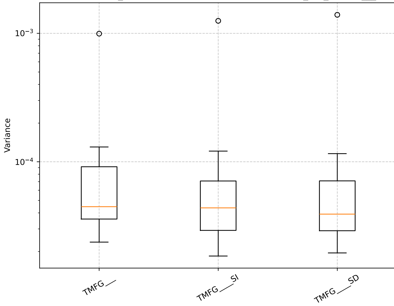
Q=1.25, len_rolling=100: Shrinkage Box Plot - min_var_, TMFG__
