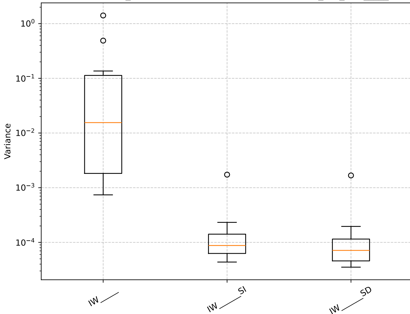
Q=1.29, len_rolling=100: Shrinkage Box Plot - min_var_, IW_____
