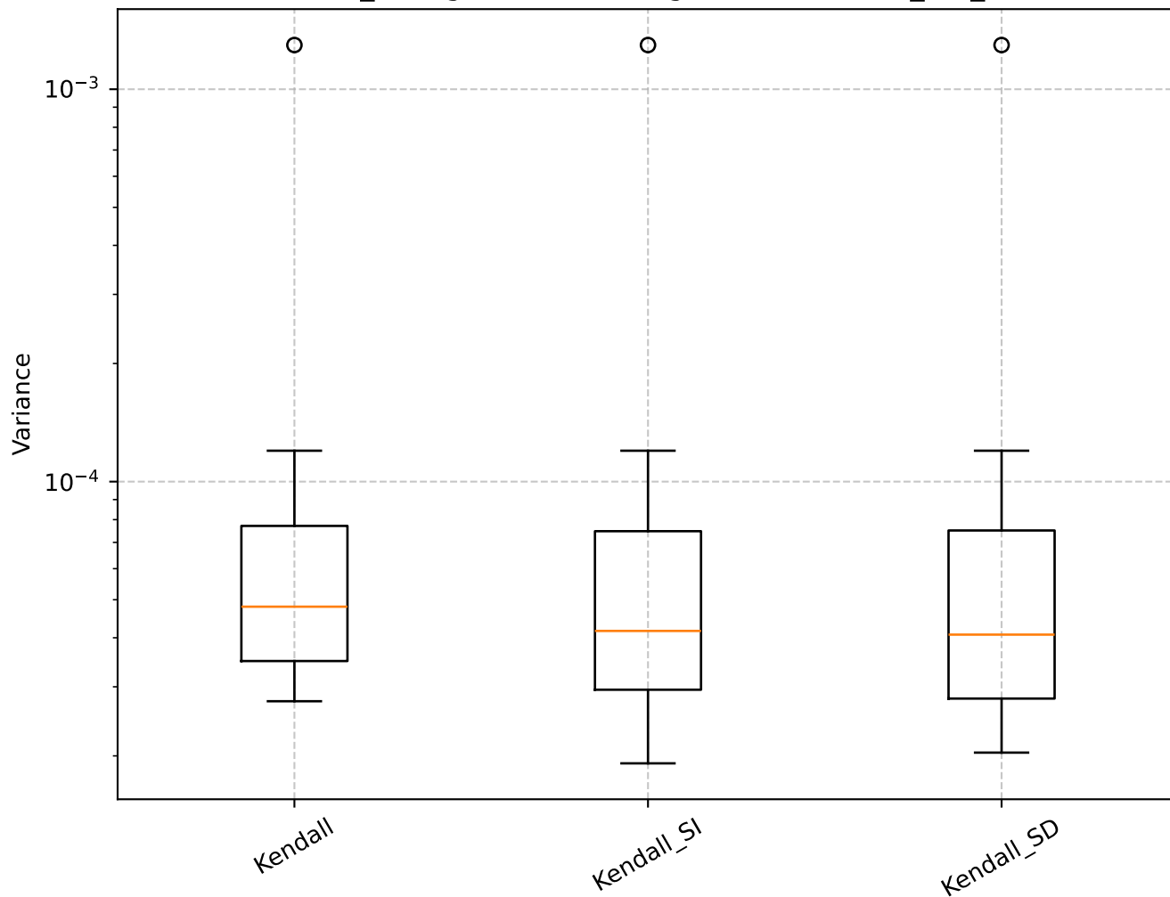
Q=1.29, len_rolling=100: Shrinkage Box Plot - min_var_, Kendall
