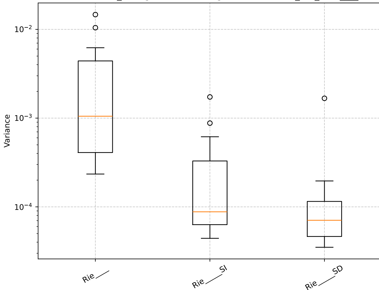
Q=1.48, len_rolling=100: Shrinkage Box Plot - min_var_, Rie__
