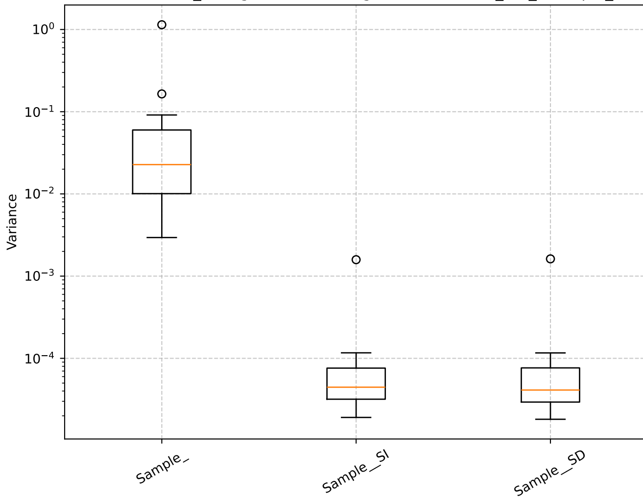
Q=1.75, len_rolling=100: Shrinkage Box Plot - min_var_, Sample_
