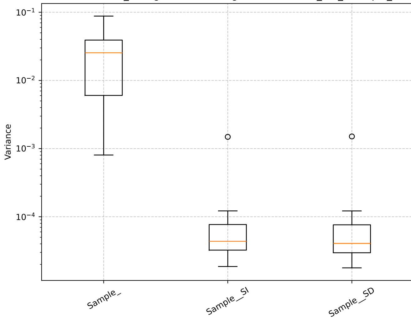
Q=1.83, len_rolling=100: Shrinkage Box Plot - min_var_, Sample_
