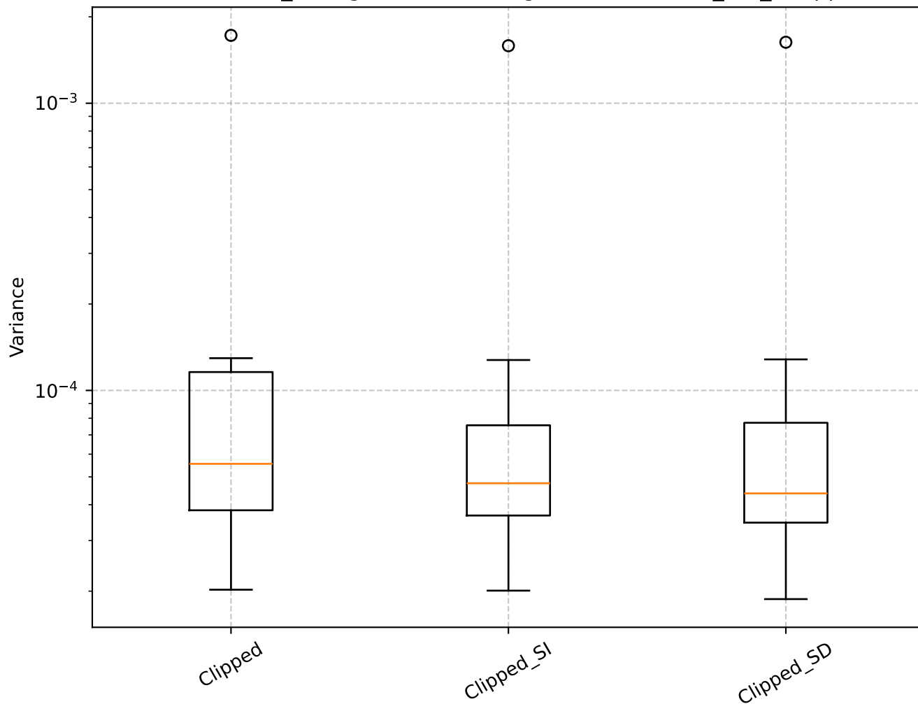
Q=1.90, len_rolling=100: Shrinkage Box Plot - min_var_, Clipped
