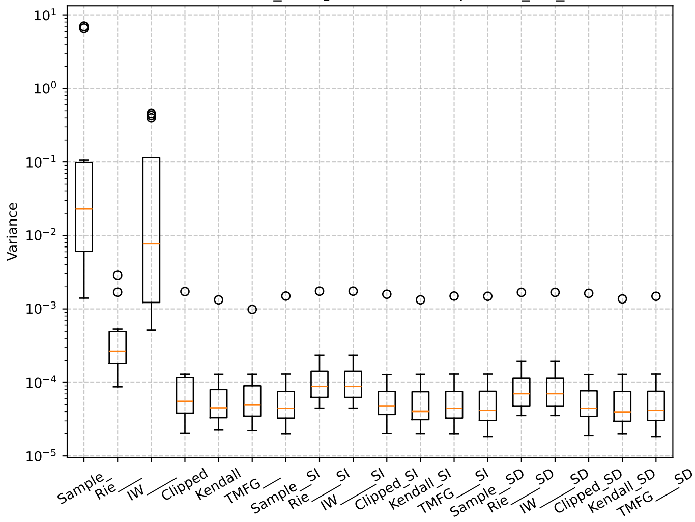
Q=1.90, len_rolling=100: Box Plot per min_var_
