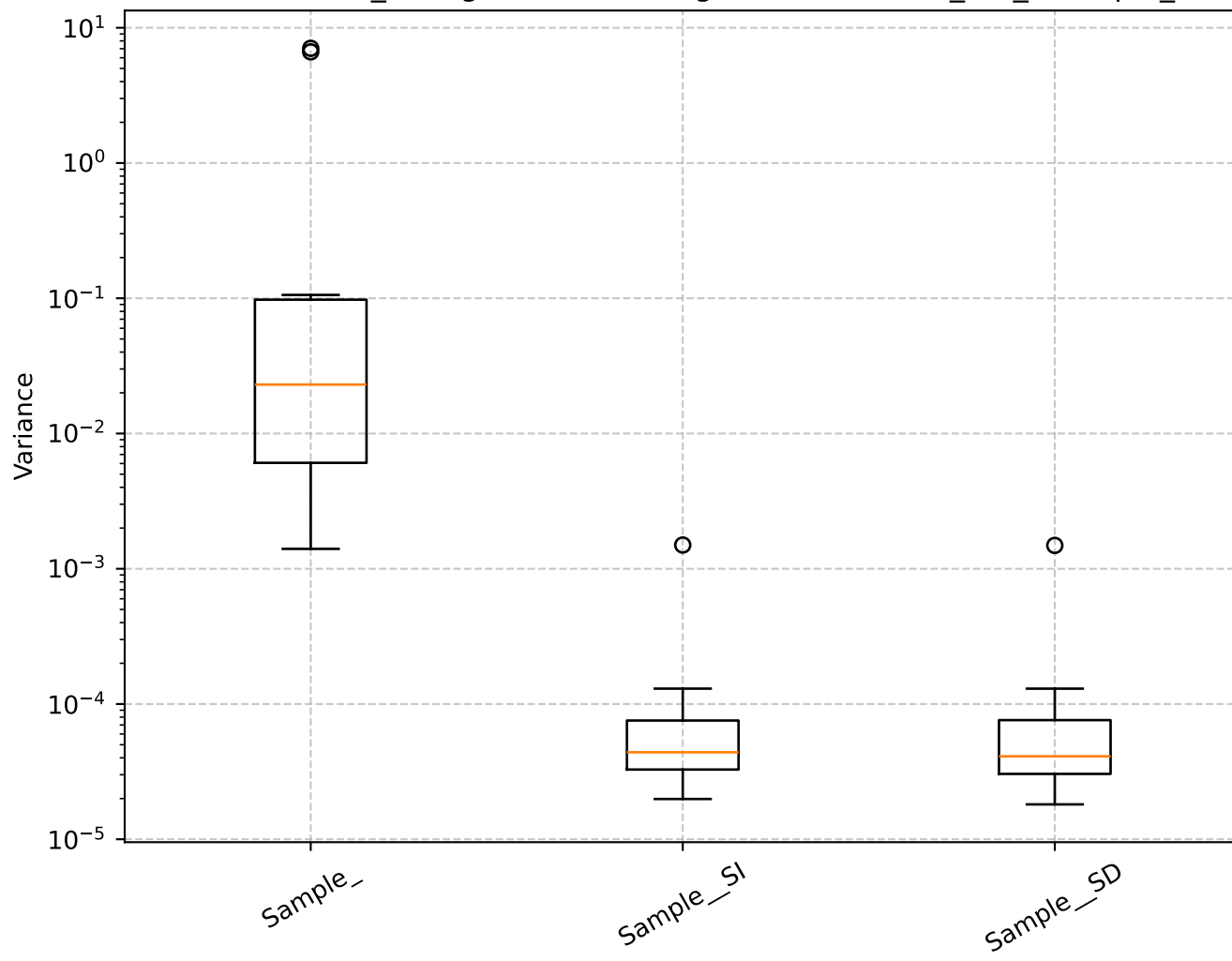
Q=1.90, len_rolling=100: Shrinkage Box Plot - min_var_, Sample_
