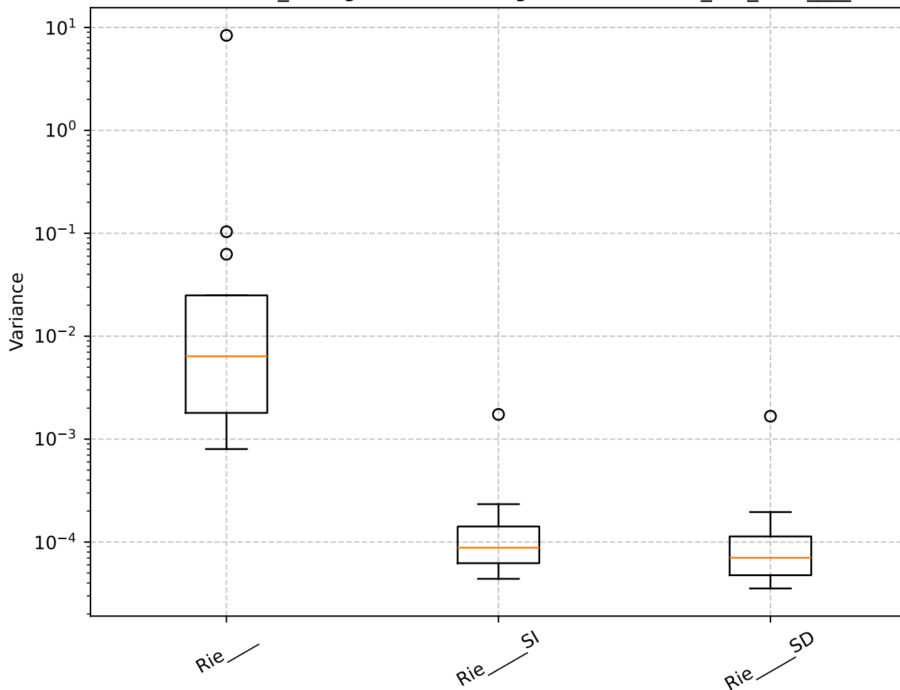
Q=2.00, len_rolling=100: Shrinkage Box Plot - min_var_, Rie_
