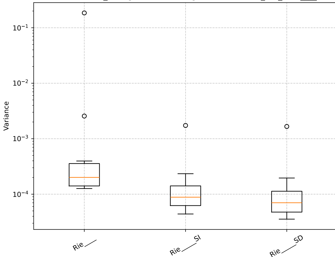
Q=2.12, len_rolling=100: Shrinkage Box Plot - min_var_, Rie_
