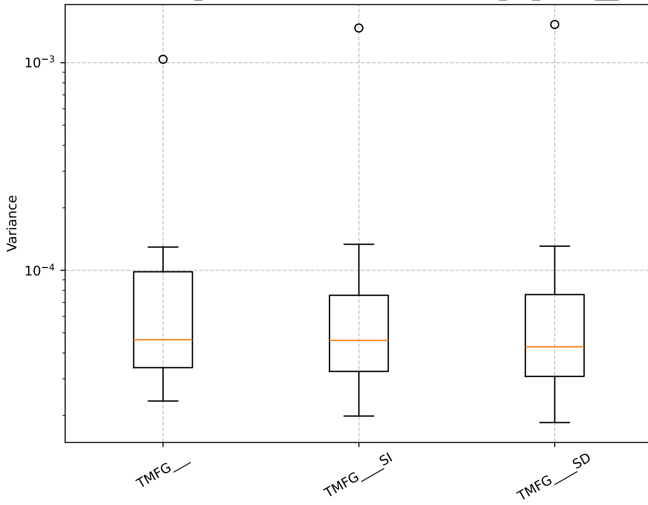
Q=2.12, len_rolling=100: Shrinkage Box Plot - min_var_, TMFG__
