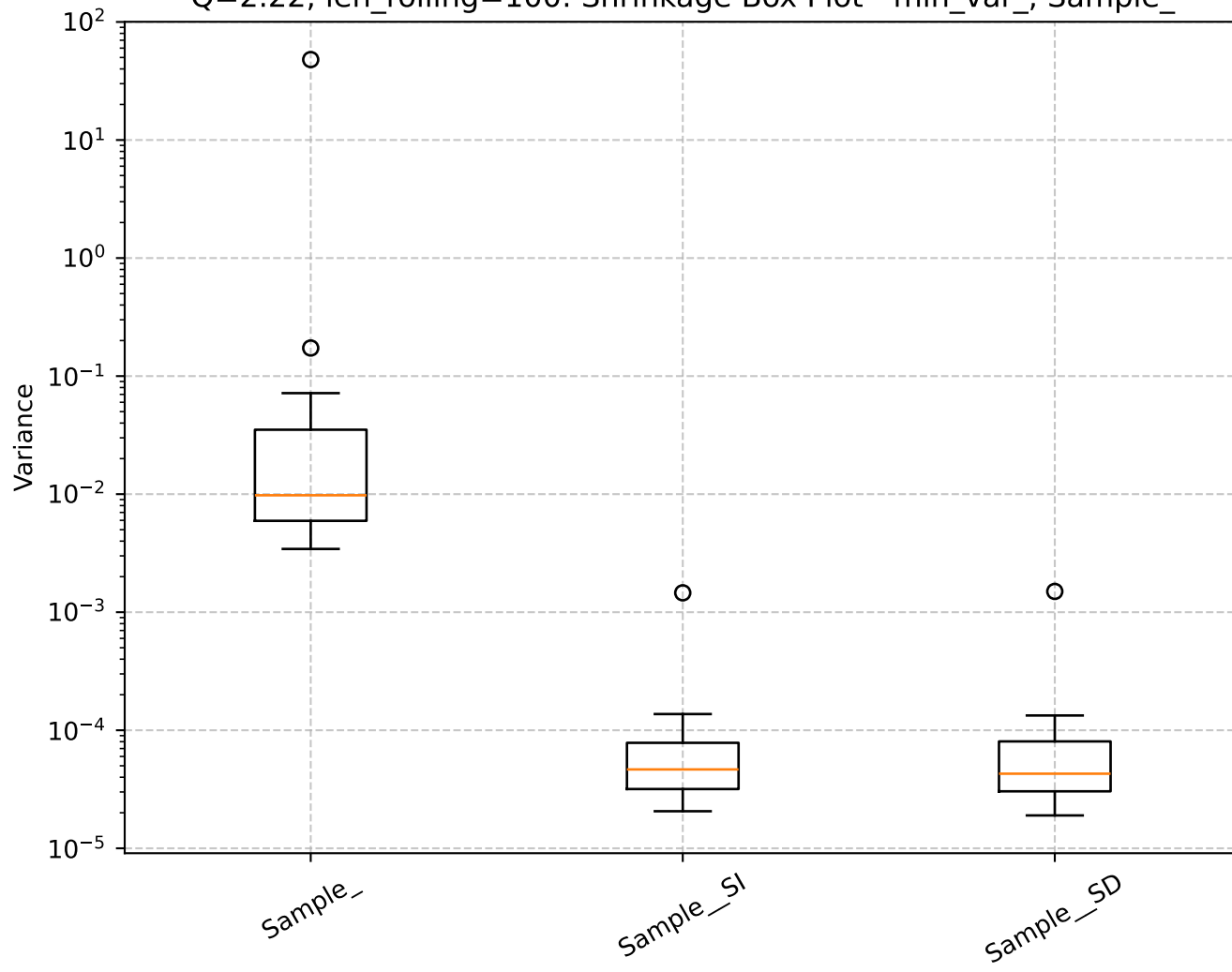
Q=2.22, len_rolling=100: Shrinkage Box Plot - min_var_, Sample_
