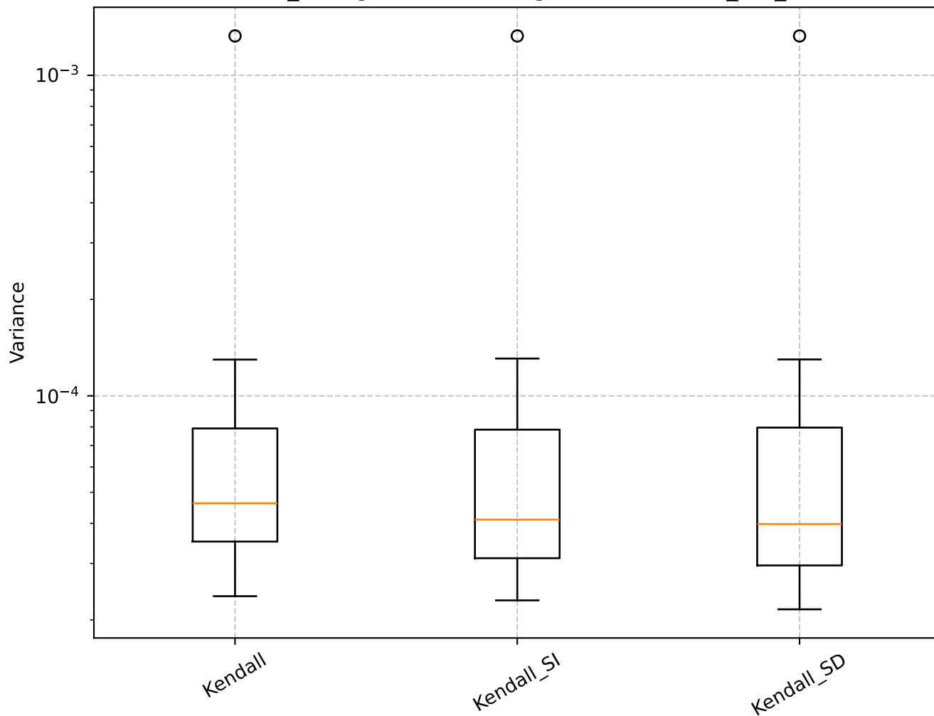
Q=2.35, len_rolling=100: Shrinkage Box Plot - min_var_, Kendall
