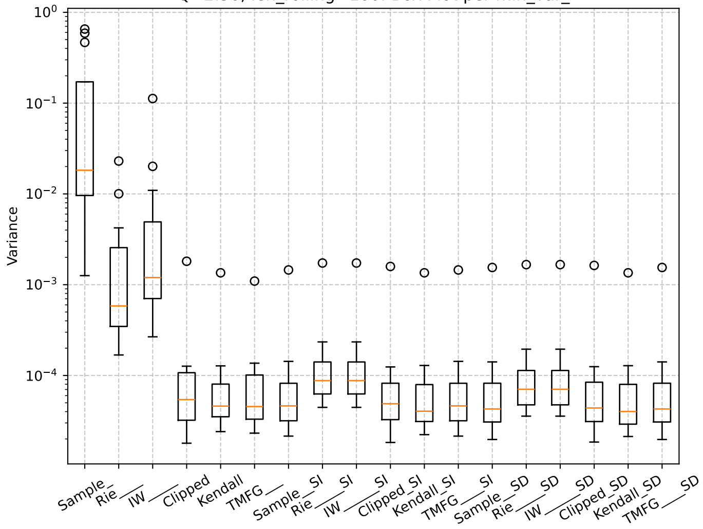
Q=2.50, len_rolling=100: Box Plot per min_var_
