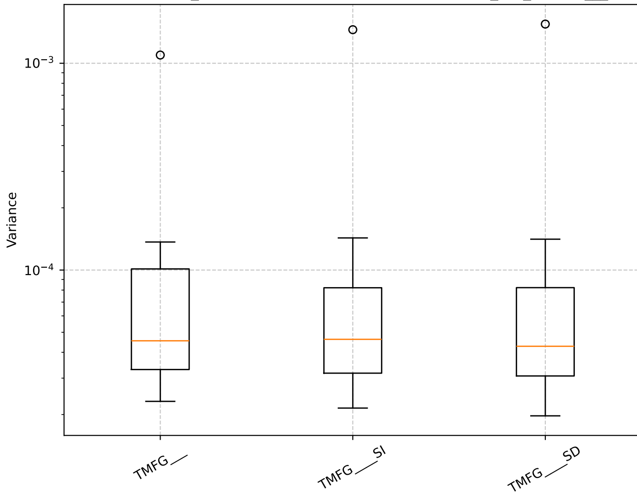
Q=2.50, len_rolling=100: Shrinkage Box Plot - min_var_, TMFG__
