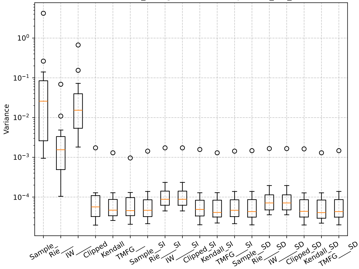
Q=2.68, len_rolling=100: Box Plot per min_var_
