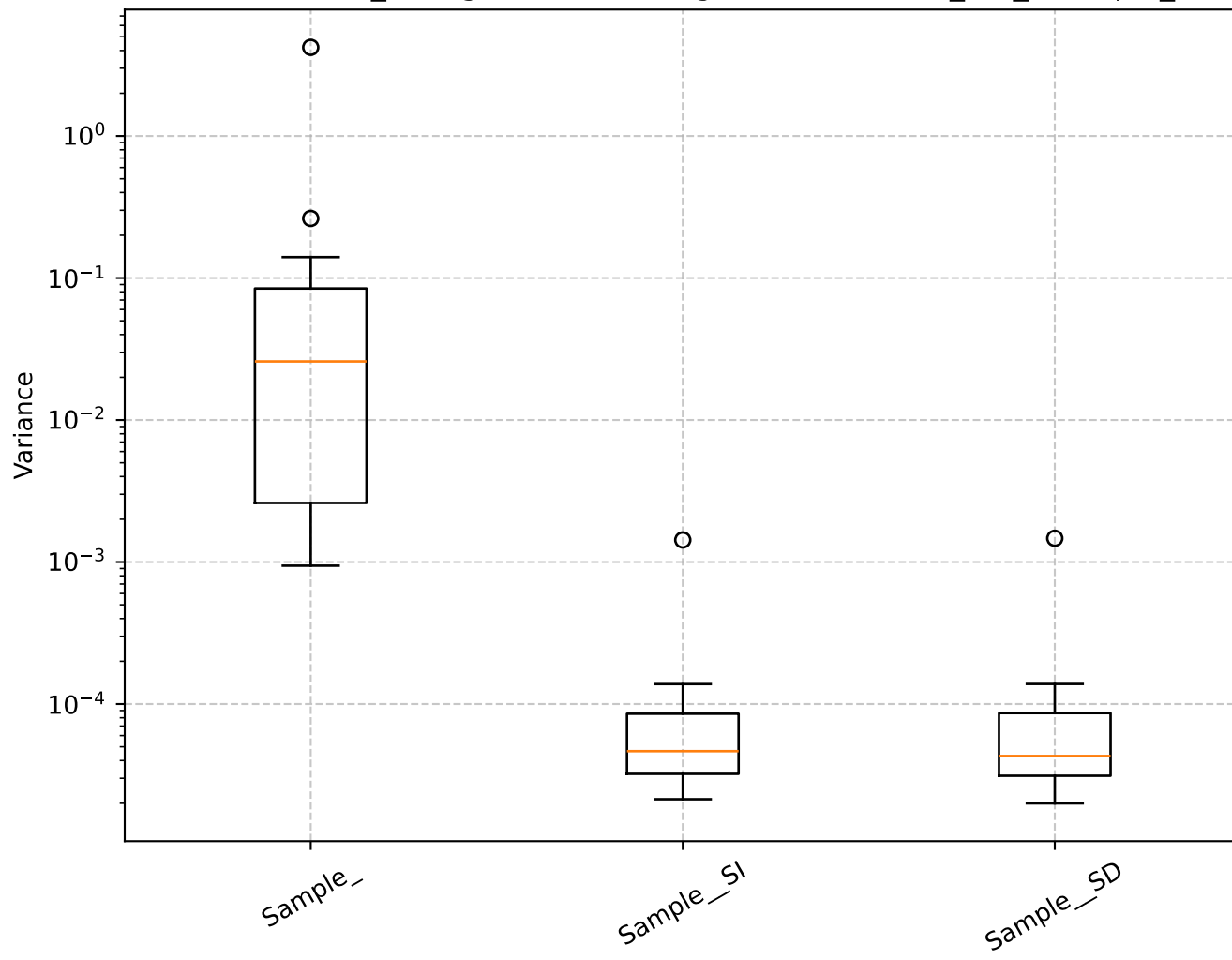
Q=2.68, len_rolling=100: Shrinkage Box Plot - min_var_, Sample_
