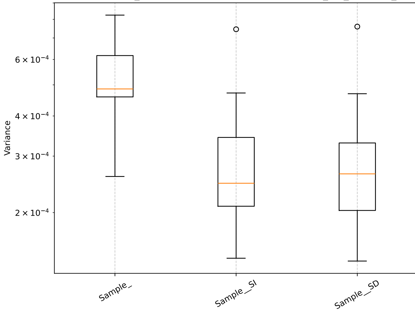
Q=0.50, len_rolling=100: Shrinkage Box Plot - min_var_, Sample_
