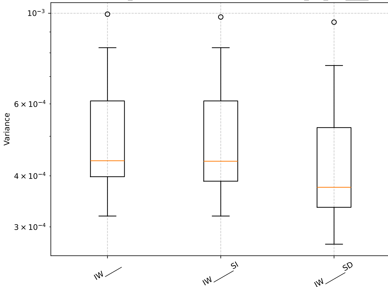
Q=0.51, len_rolling=100: Shrinkage Box Plot - min_var_, IW_____
