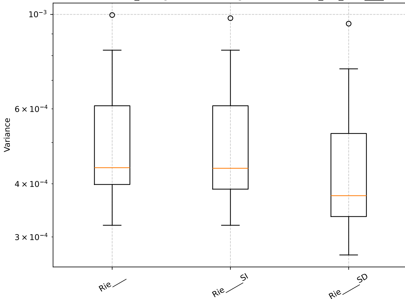
Q=0.51, len_rolling=100: Shrinkage Box Plot - min_var_, Rie__
