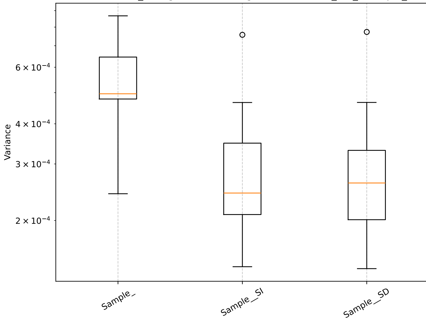
Q=0.51, len_rolling=100: Shrinkage Box Plot - min_var_, Sample_
