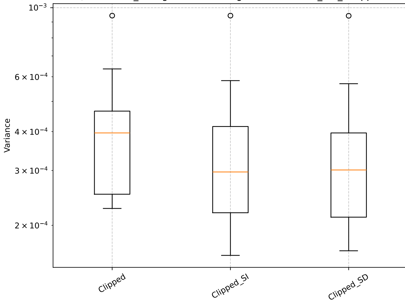
Q=0.53, len_rolling=100: Shrinkage Box Plot - min_var_, Clipped
