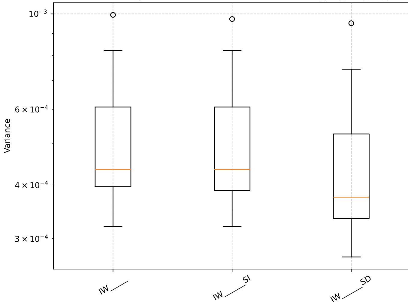
Q=0.53, len_rolling=100: Shrinkage Box Plot - min_var_, IW_____
