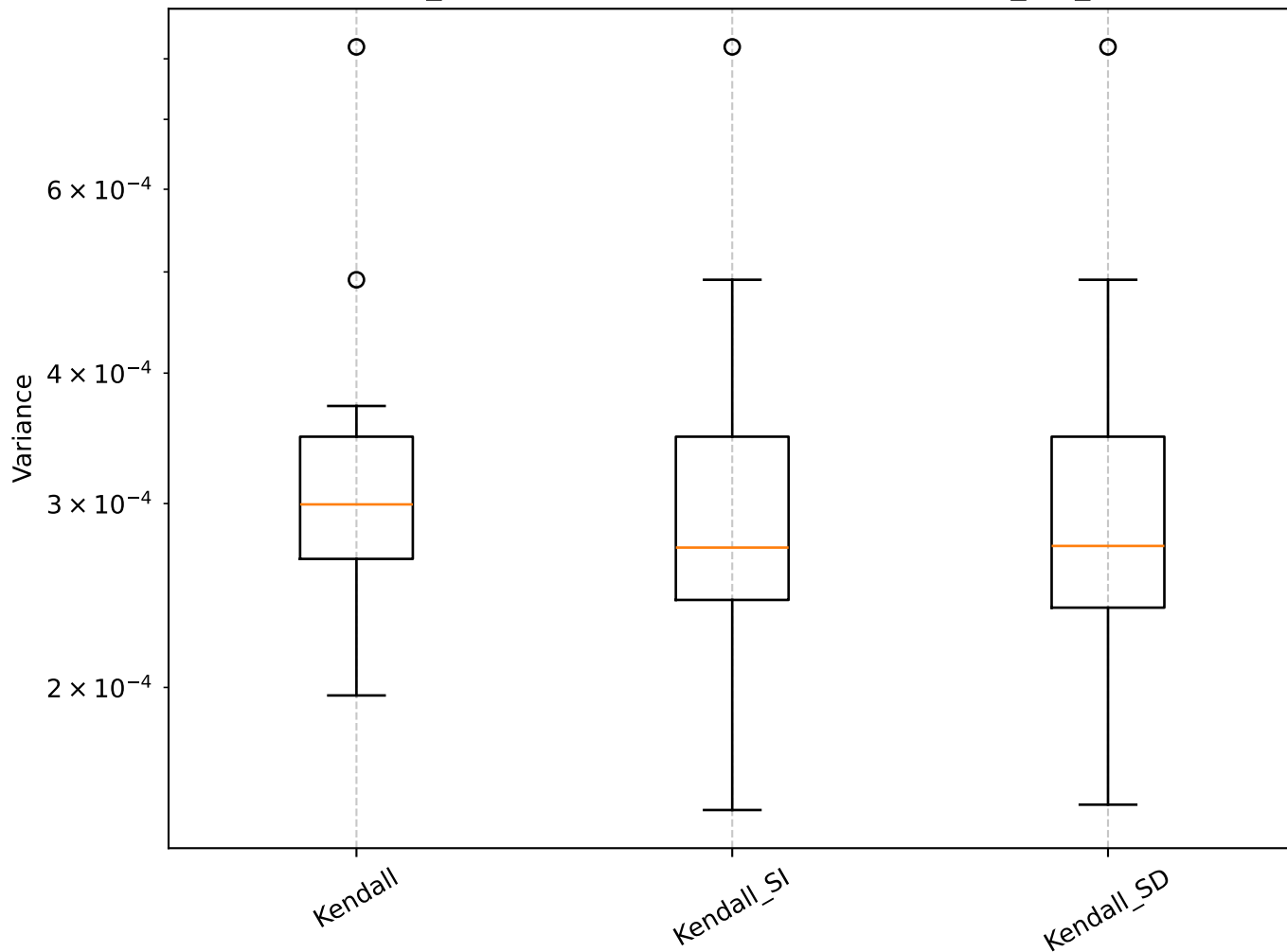
Q=0.53, len_rolling=100: Shrinkage Box Plot - min_var_, Kendall
