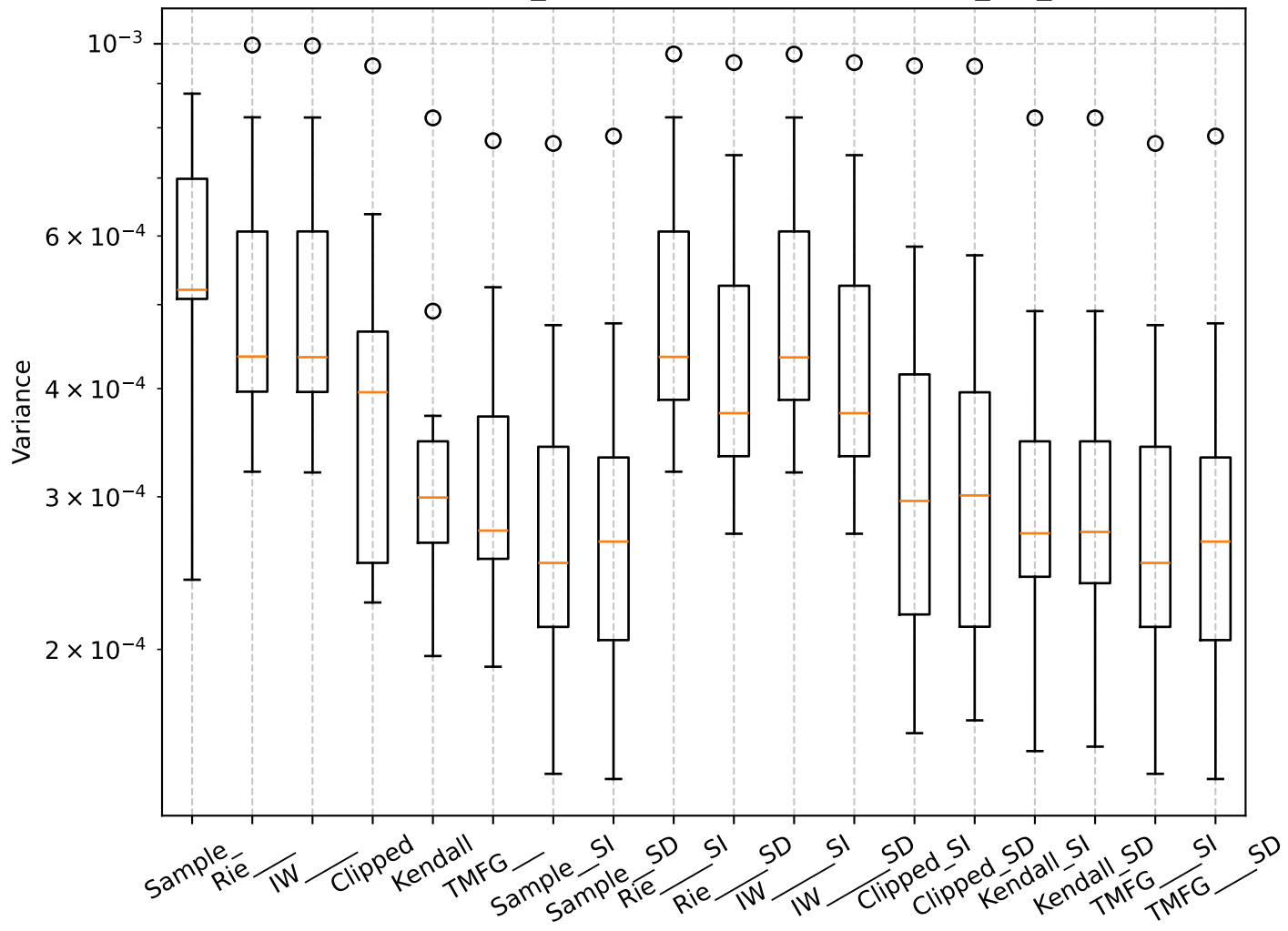
Q=0.53, len_rolling=100: Box Plot per min_var
