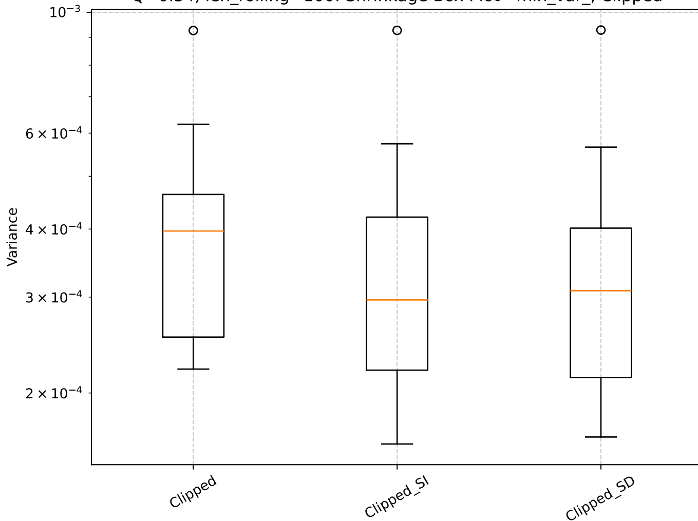
Q=0.54, len_rolling=100: Shrinkage Box Plot - min_var_, Clipped
