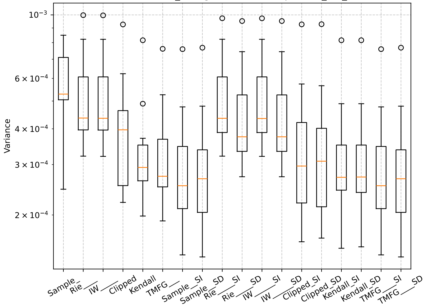
Q=0.54, len_rolling=100: Box Plot per min_var_
