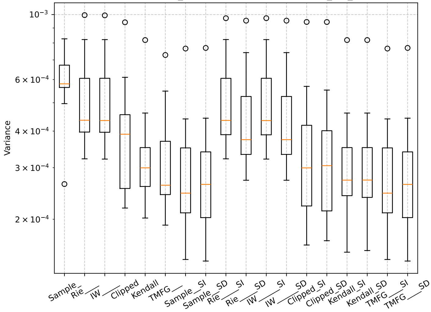
Q=0.56, len_rolling=100: Box Plot per min_var_
