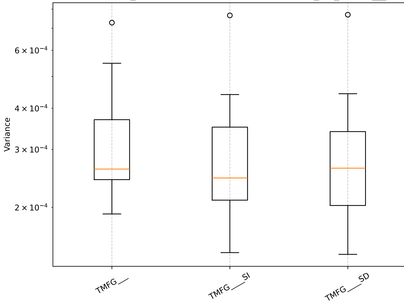
Q=0.56, len_rolling=100: Shrinkage Box Plot - min_var_, TMFG__
